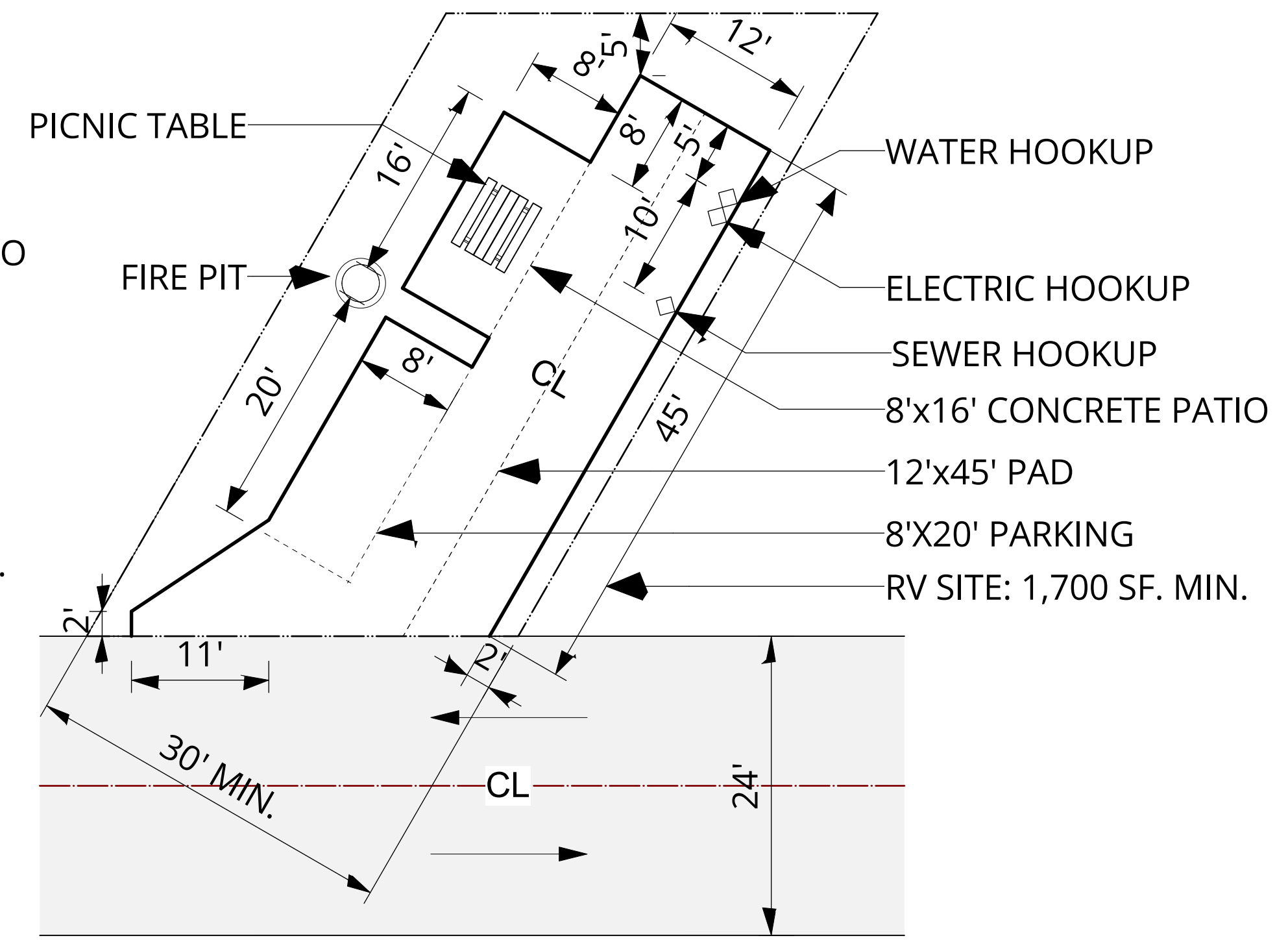
45' BACK-IN NOT TO SCALE
