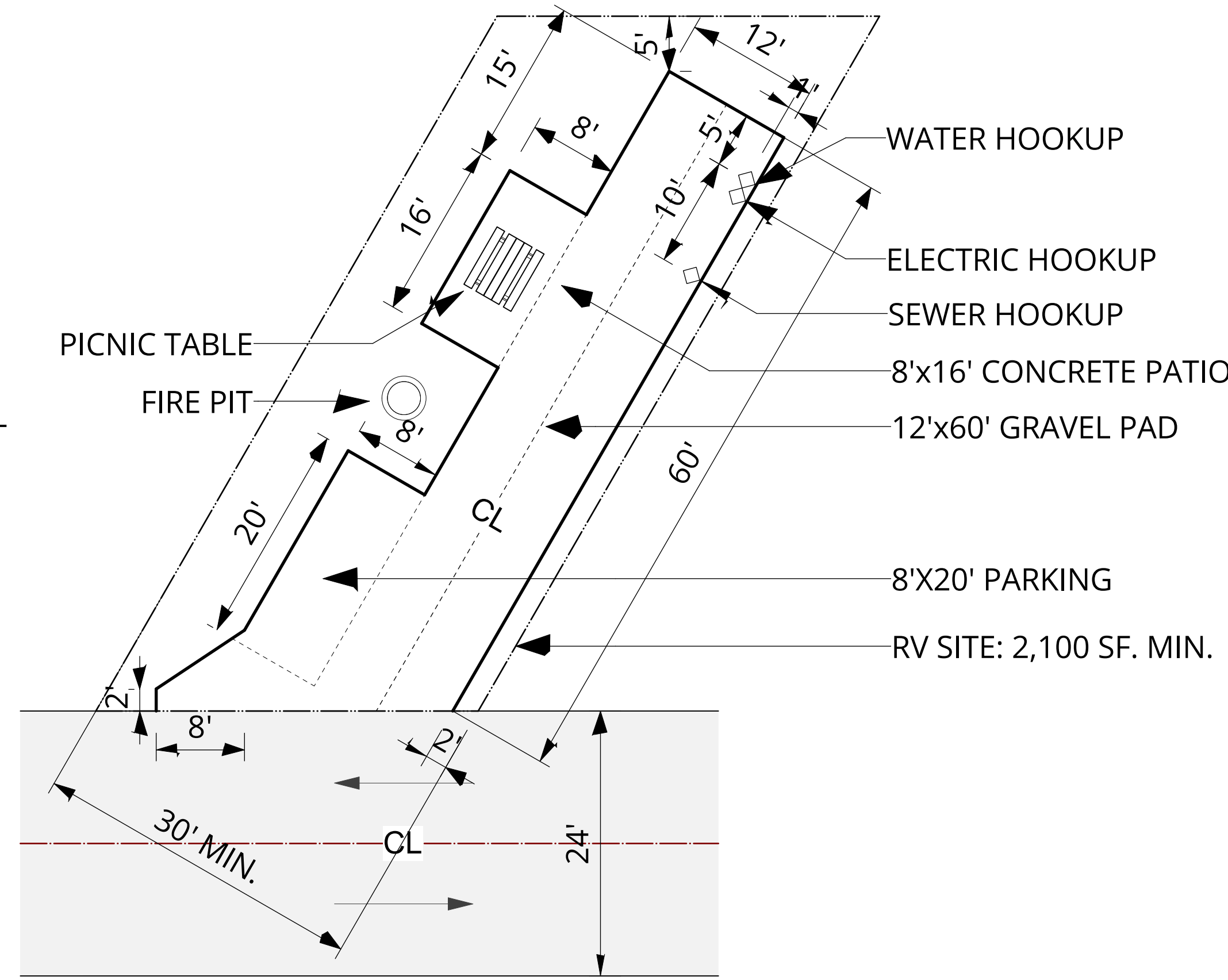
60' BACK-IN NOT TO SCALE
