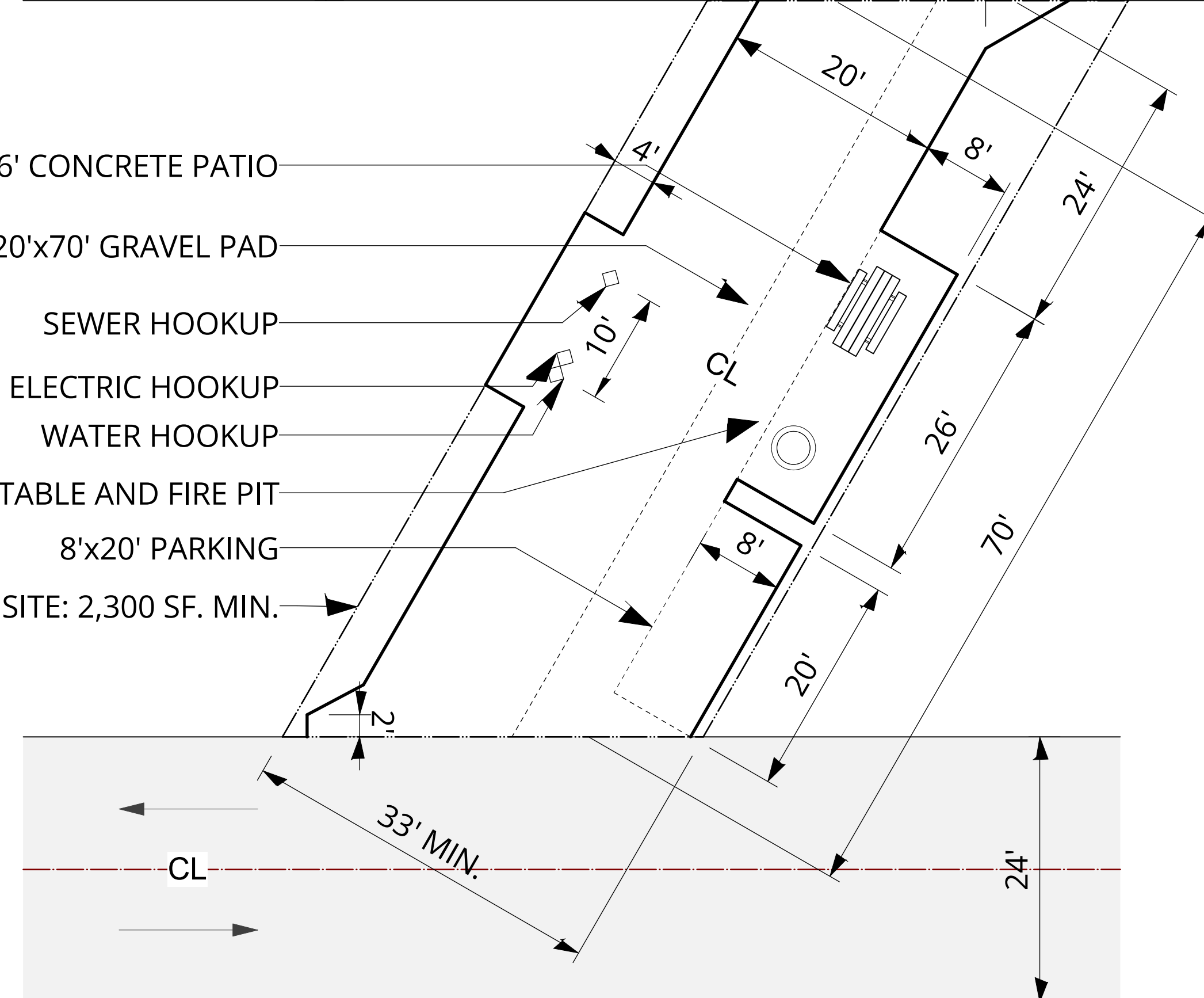
ADA PULL-THRU NOT TO SCALE
