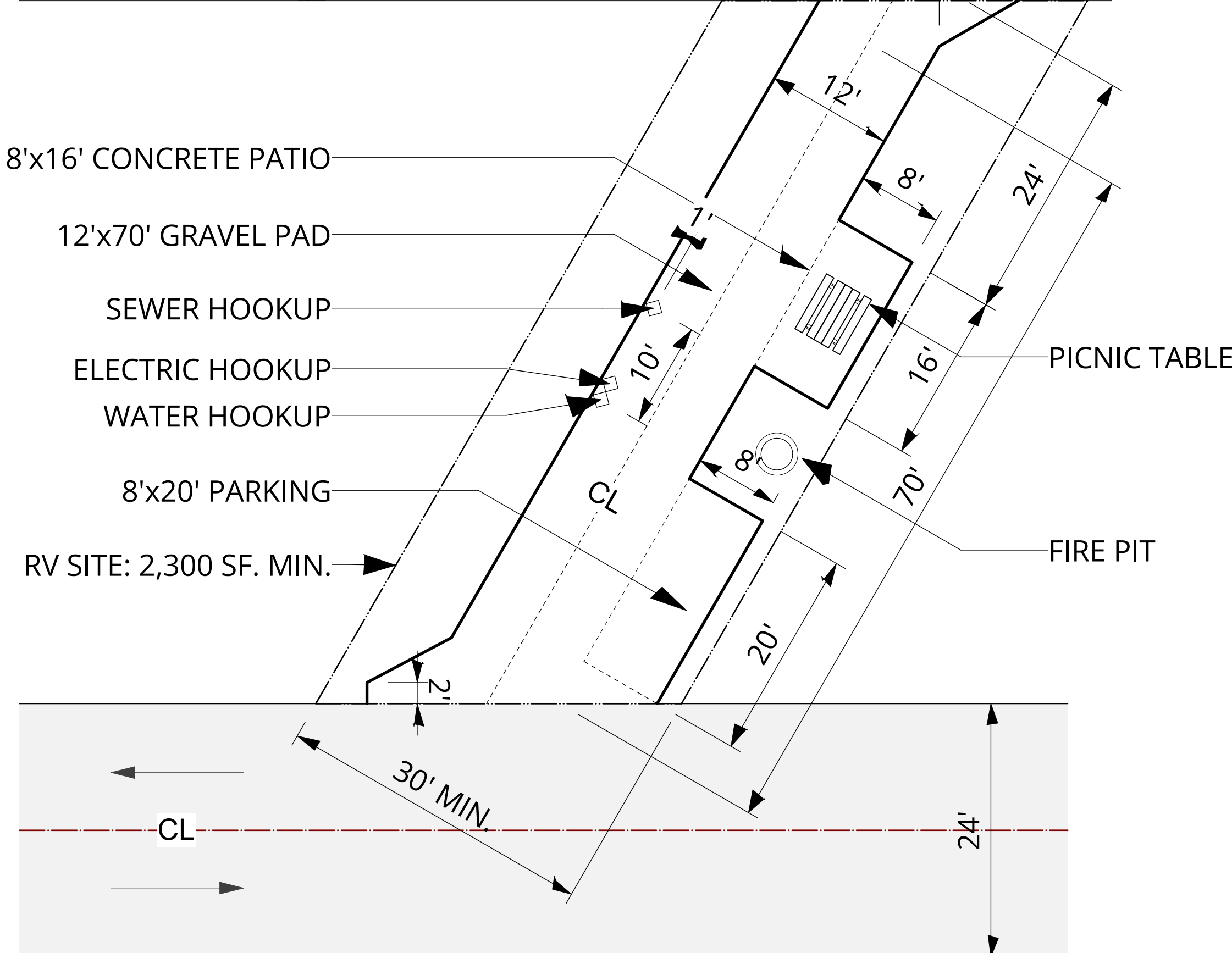
PULL-THRU NOT TO SCALE
