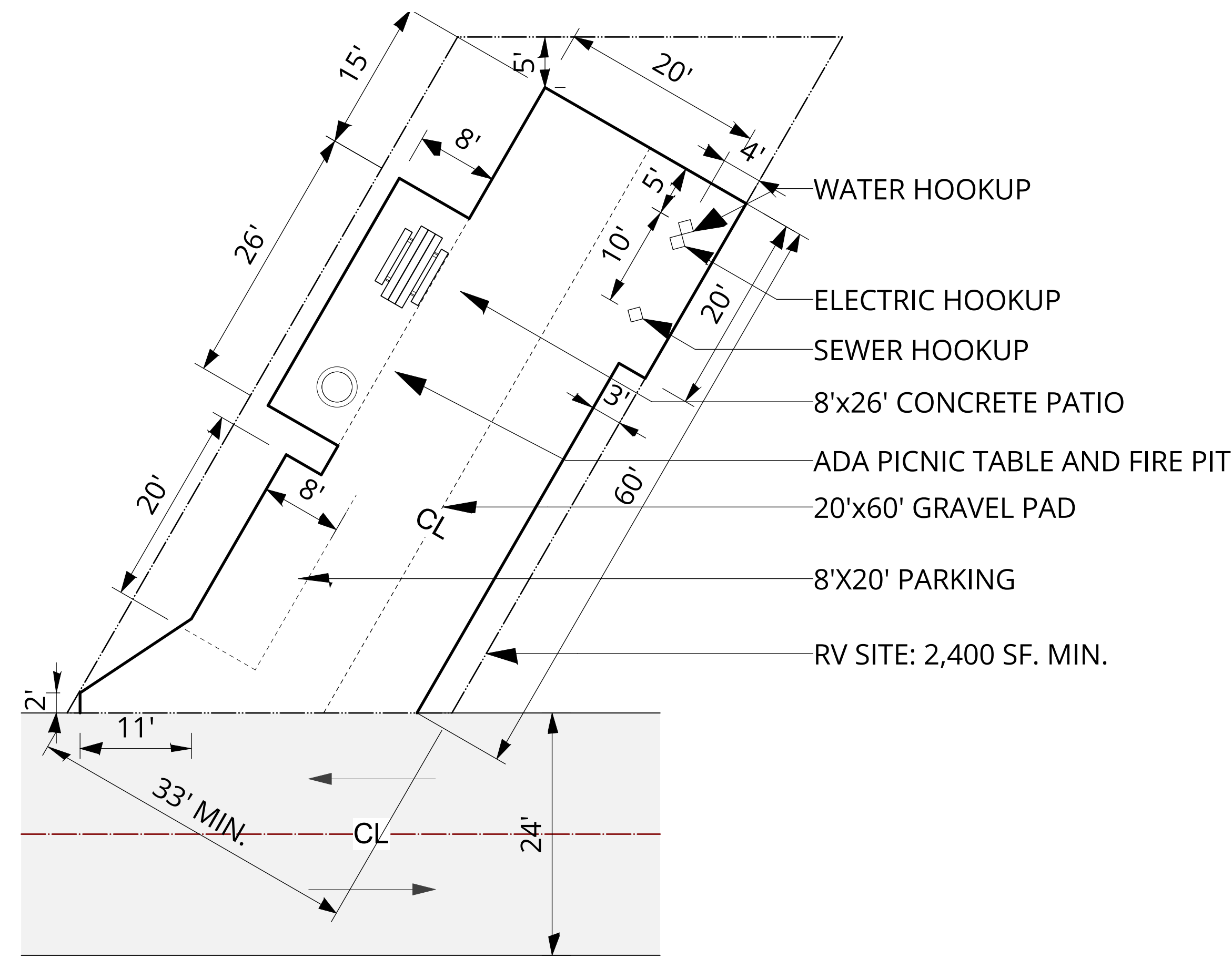
ADA BACK-IN NOT TO SCALE
